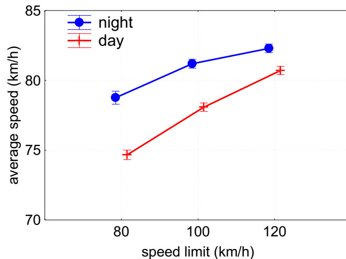
Figure 3.3: Average speed of trucks on roads with different speed limits during day and night (Hogema, 2009).
