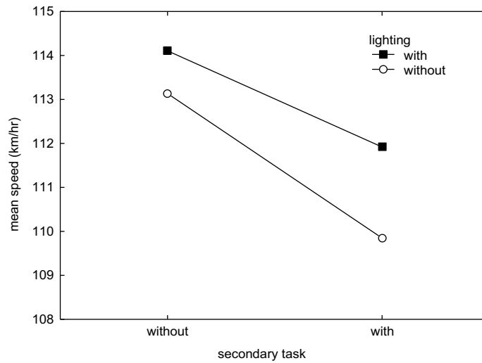
Figure 3.2: Average speed on a motorway with or without lighting and while performing a secondary task or not (Hogema et. al. 2005).
